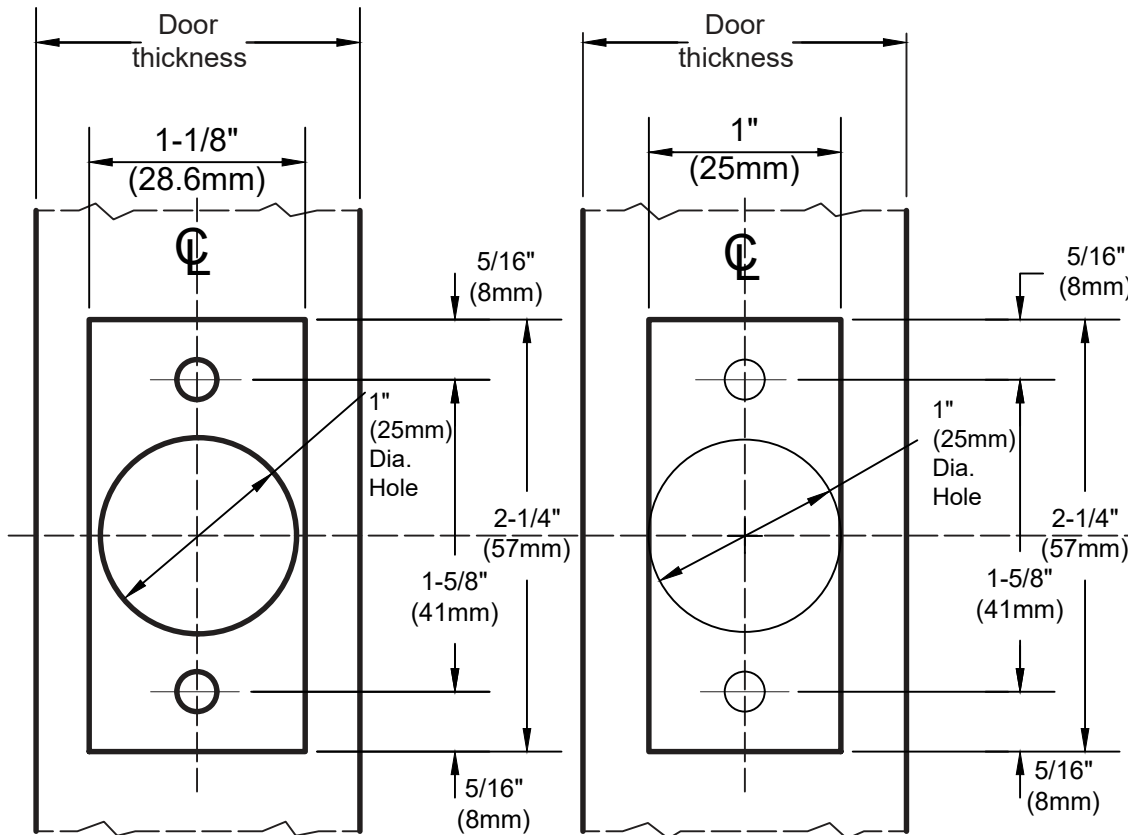
Standard 2-3/4" Latch
